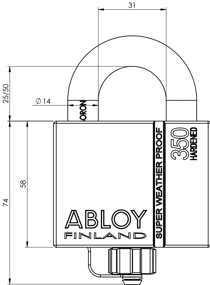
PLM350T
